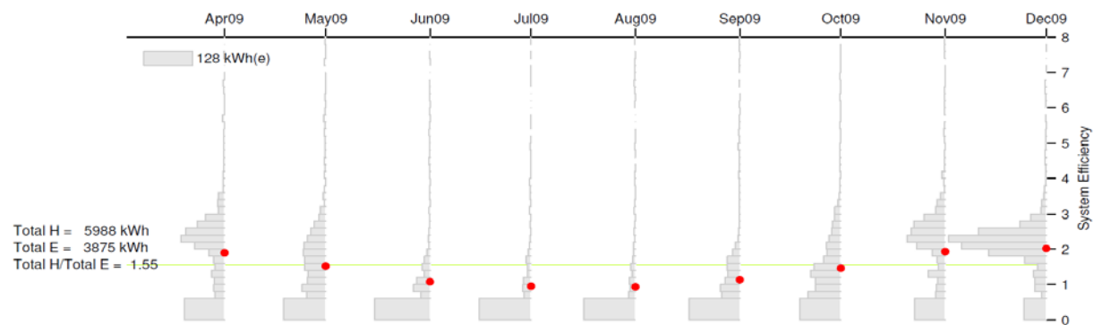
Figure 30: Monthly distribution of system efficiencies (site 487)
