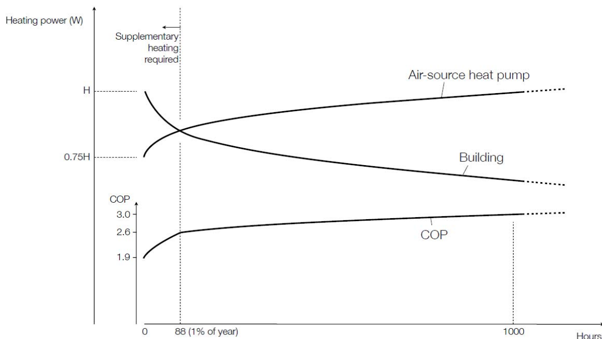
Figure 42: A schematic of a load duration curve for an air-source heat pump
