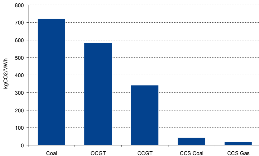
Figure 11 – Carbon dioxide emissions by generating type
