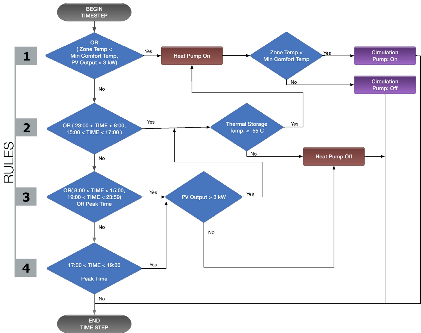
Fig. 2. Algorithm diagram flow chart.
